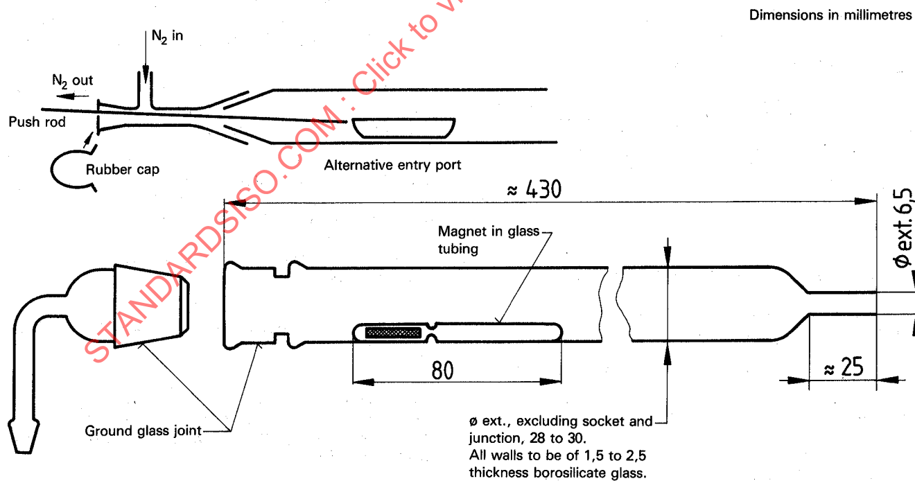
Figure 2 — Drying tube (5.3)
