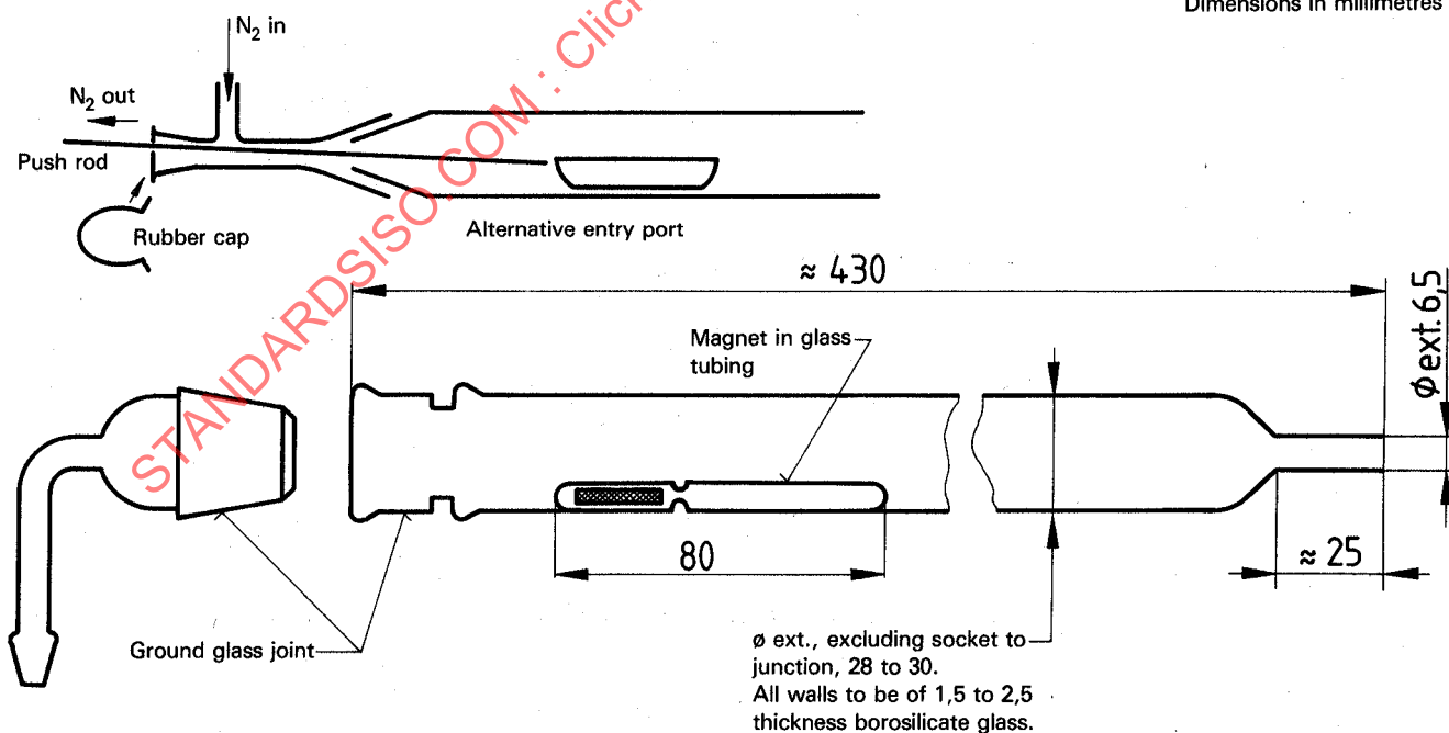
Figure 4 — Drying tube (11.2)
