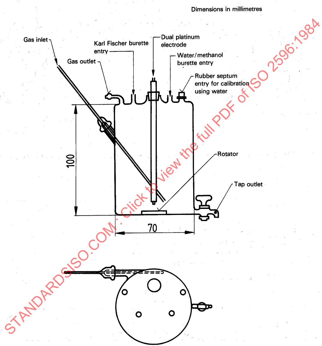
Figure 5 — Absorption cell (11.9)
