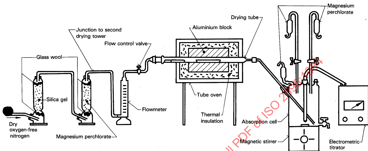
Figure 3 — Apparatus for the determination of hygroscopic moisture — Method 2 (Karl Fischer method)
