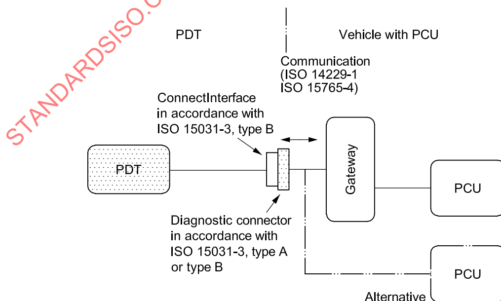
Figure 1 — Access to the vehicle via diagnostic connector
