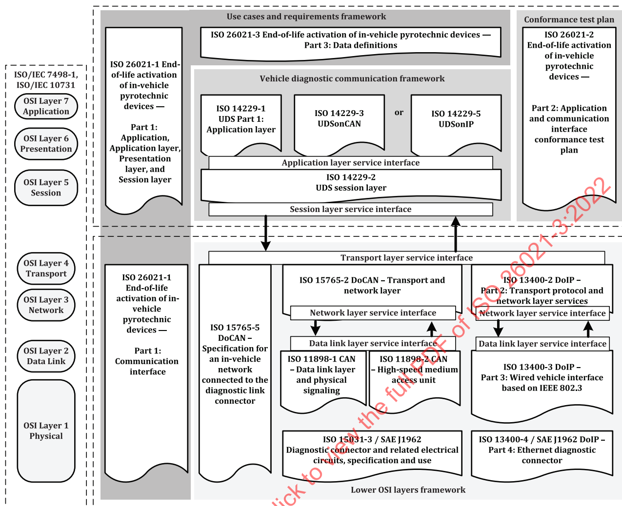
Figure 1 — ISO 26021 documents reference according to OSI model
