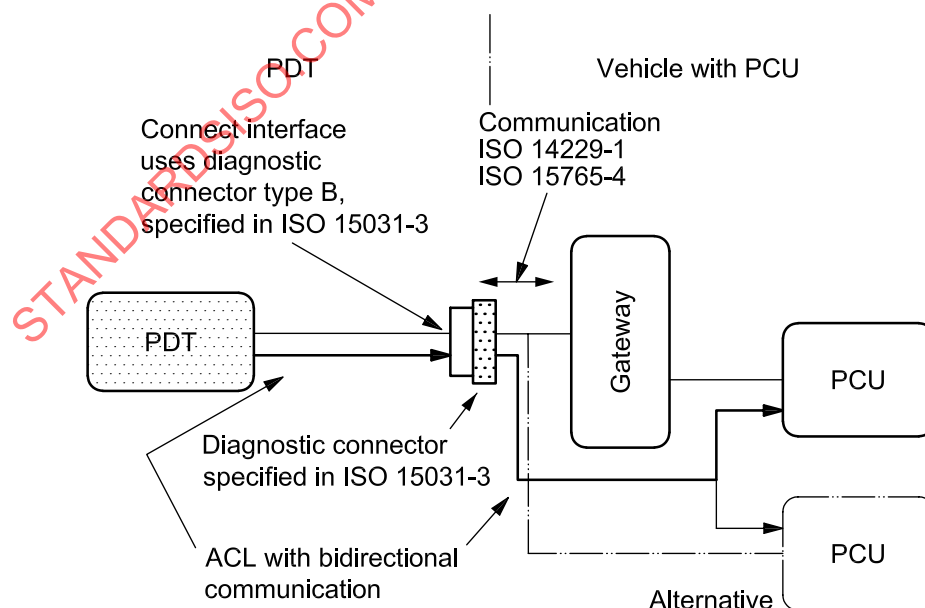
Figure 1 — Access to the vehicle via diagnostic connector
