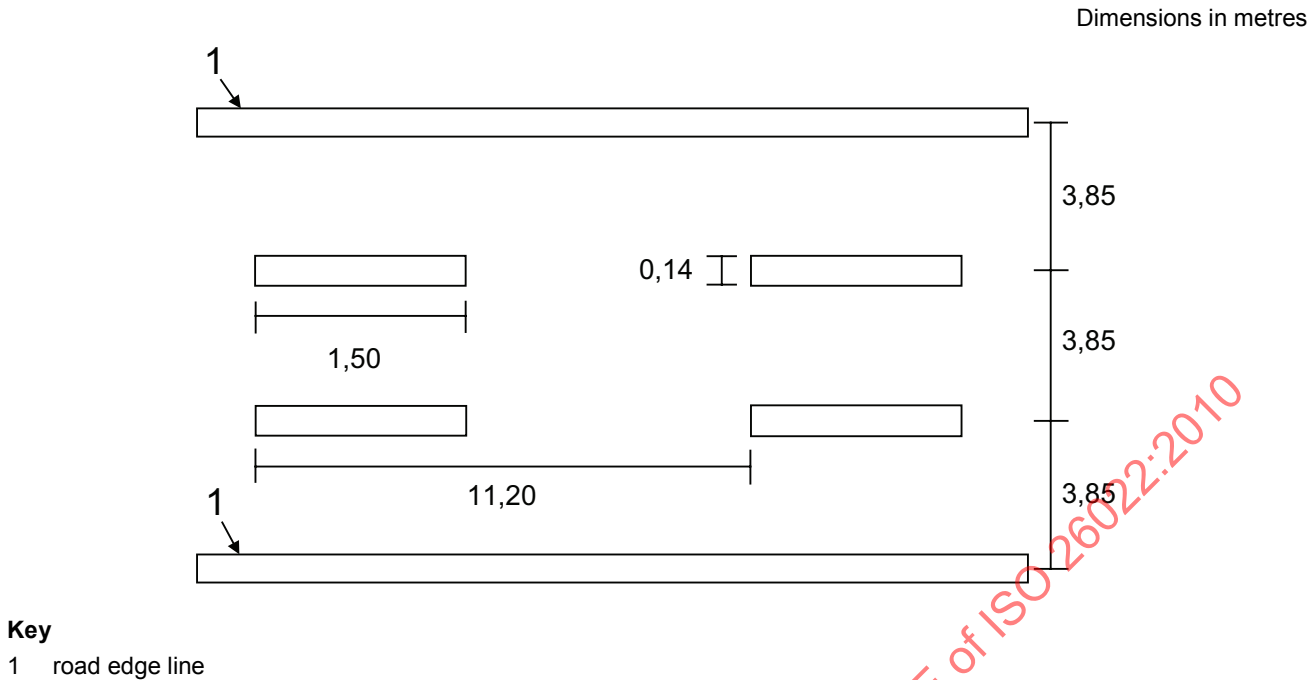
Figure 2 — Dimensions of the road markers (not to scale)
