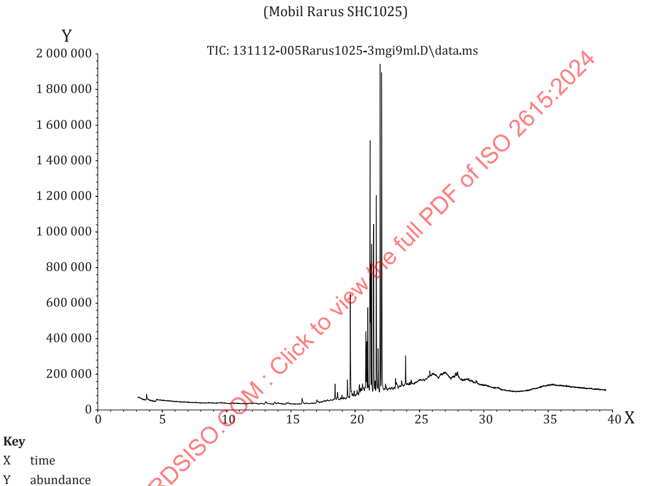
Figure A.1 — Chromatogram of a compressor oil with indication of the retention time in minutes
