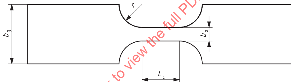
Figure 1 — Type-A test piece
