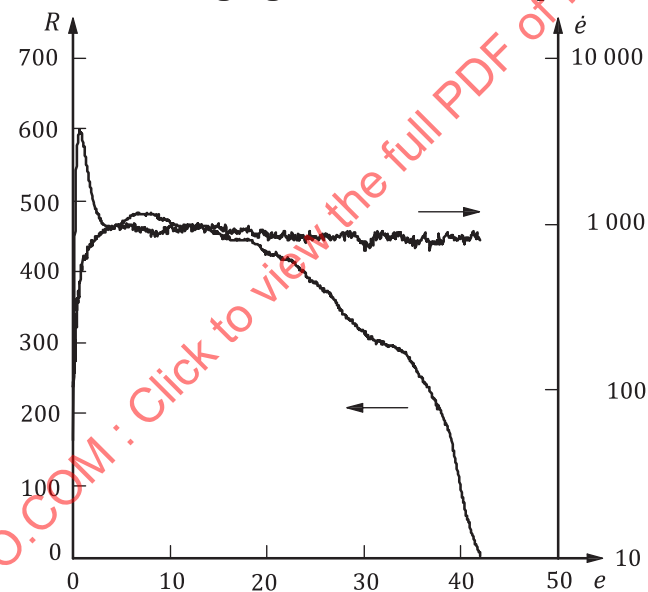
b) Engineering stress, engineering strain and engineering strain rate obtained by analysis of raw data
