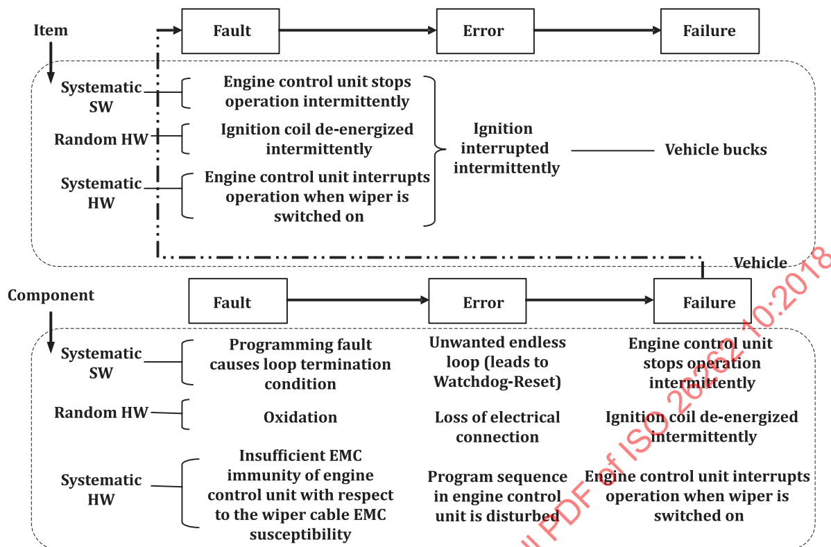
Figure 5 — Example of faults leading to failures
