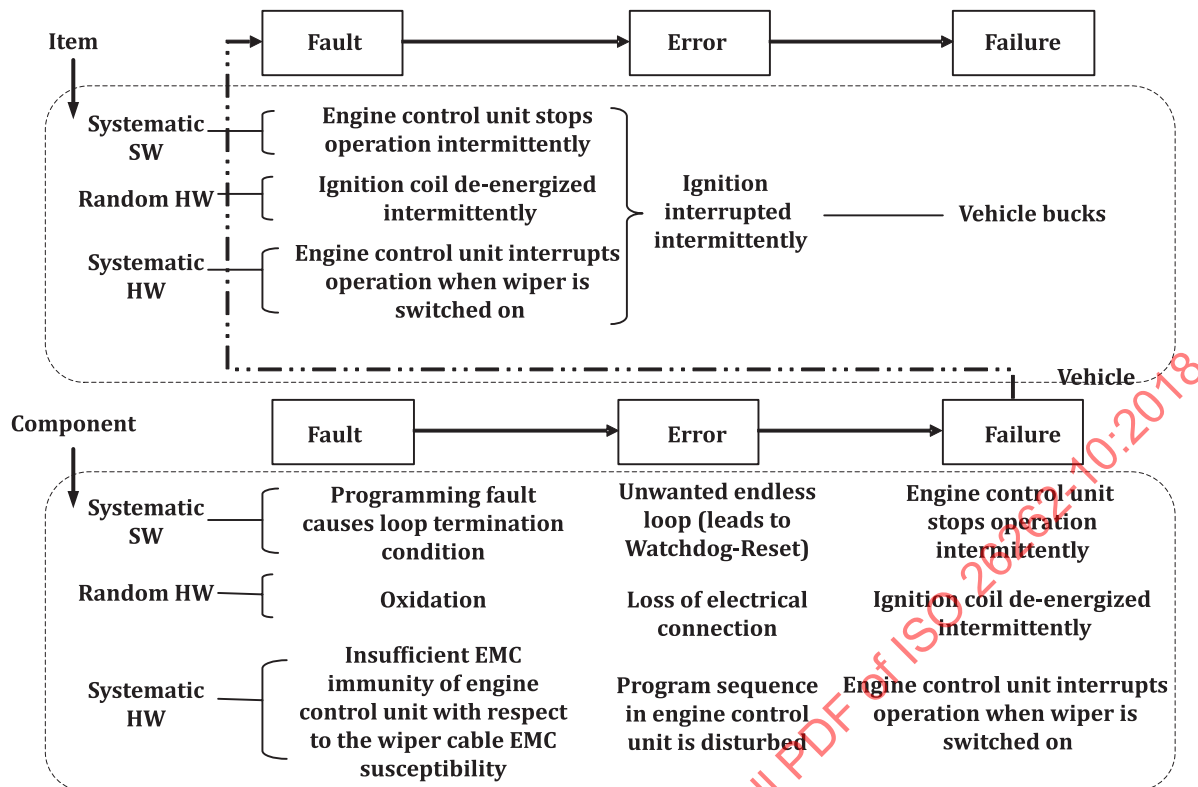
Figure 5 — Example of faults leading to failures
