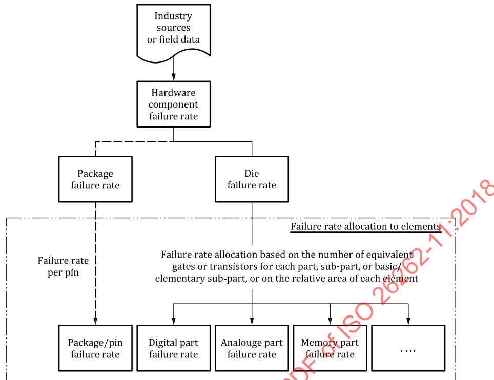
Figure 19 — Failure rate distribution
