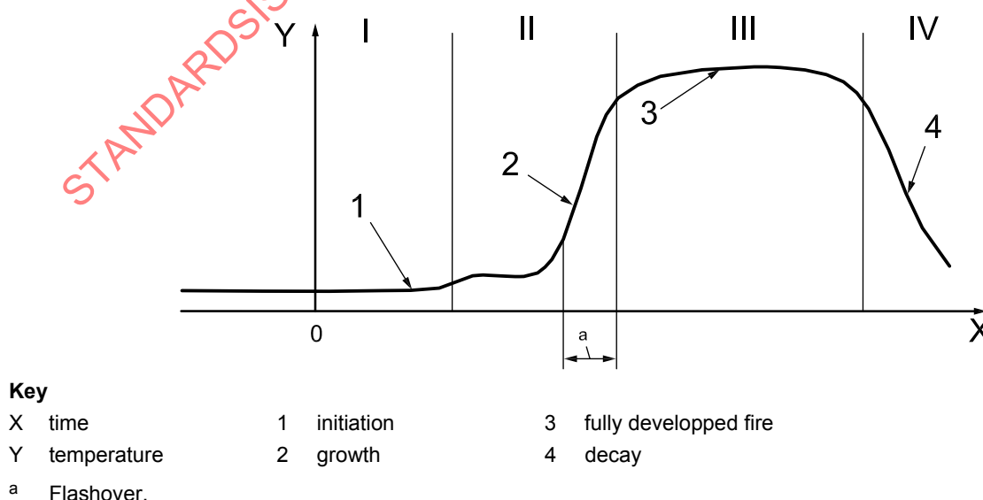
Figure 2 — Potential fire development in an enclosure
