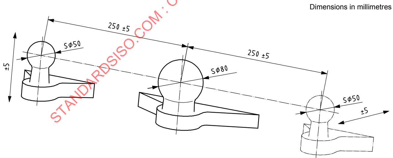
Figure 3 — Location of connecting point(s) of tractor (50 mm ball) in relation to 80 mm ball-type coupling device
