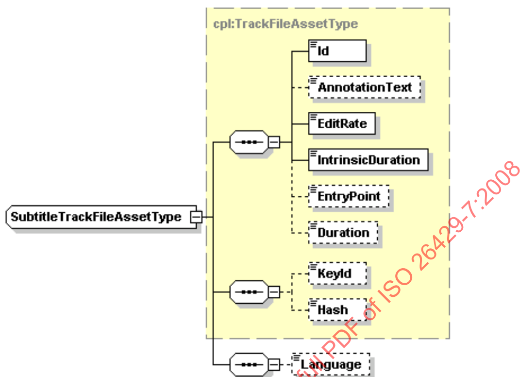
Figure 15 – Subtitle Track File Asset structure (Dotted lines denote an optional element)
