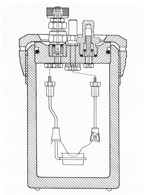
Figure 1 — Parr oxygen bomb
