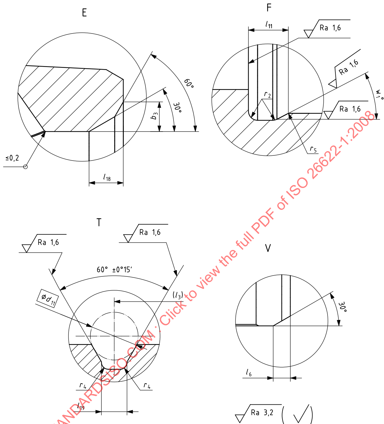
Figure 1 — Tapered hollow shank
