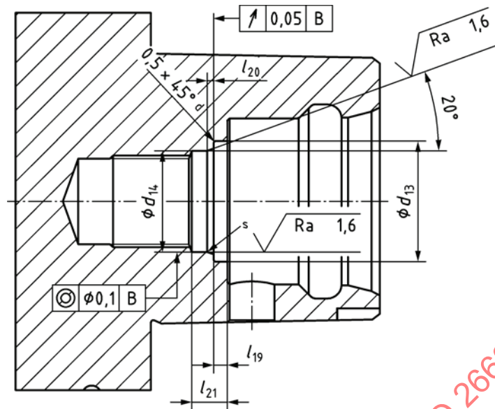
Size 100 polygon shanks
