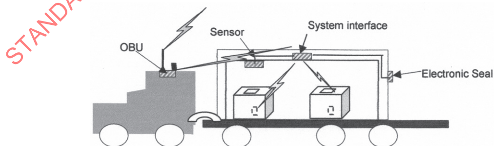
Figure 3 — Tractor with one trailer with cargo on it
