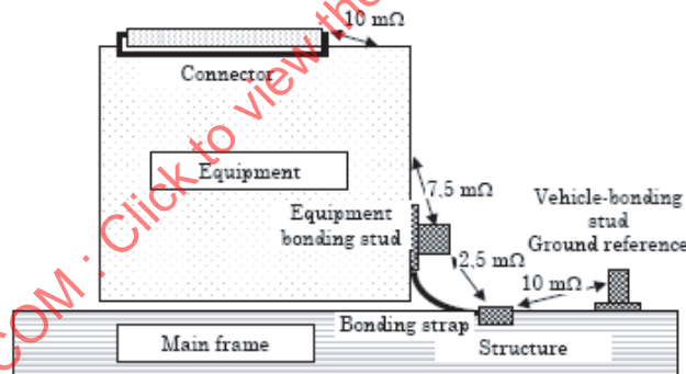
Figure 2 — Bonding requirements
