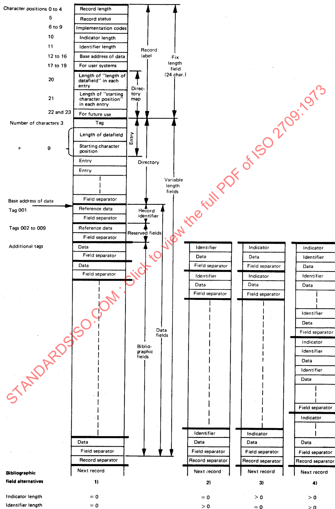
FIGURE 2 – Detailed structure
