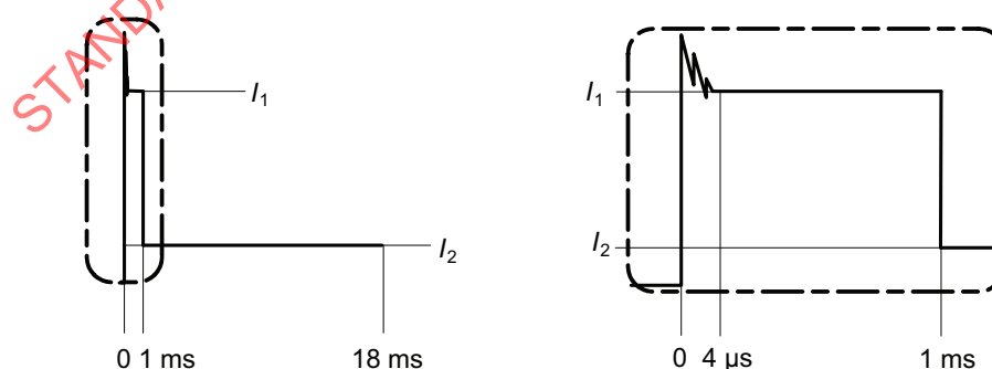
Figure C.3 — Leakage current waveform
