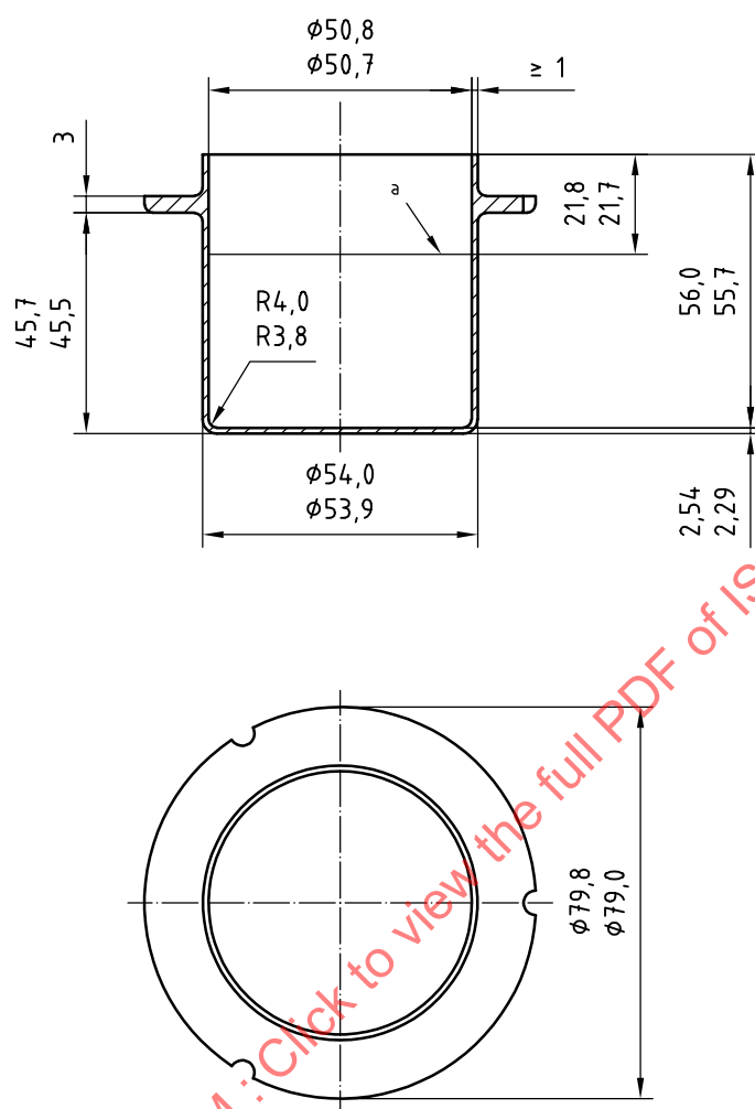
Figure B.2 — Test cup
