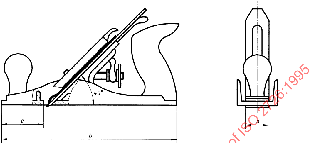
Figure 2 — Metal-bodied bench planes
