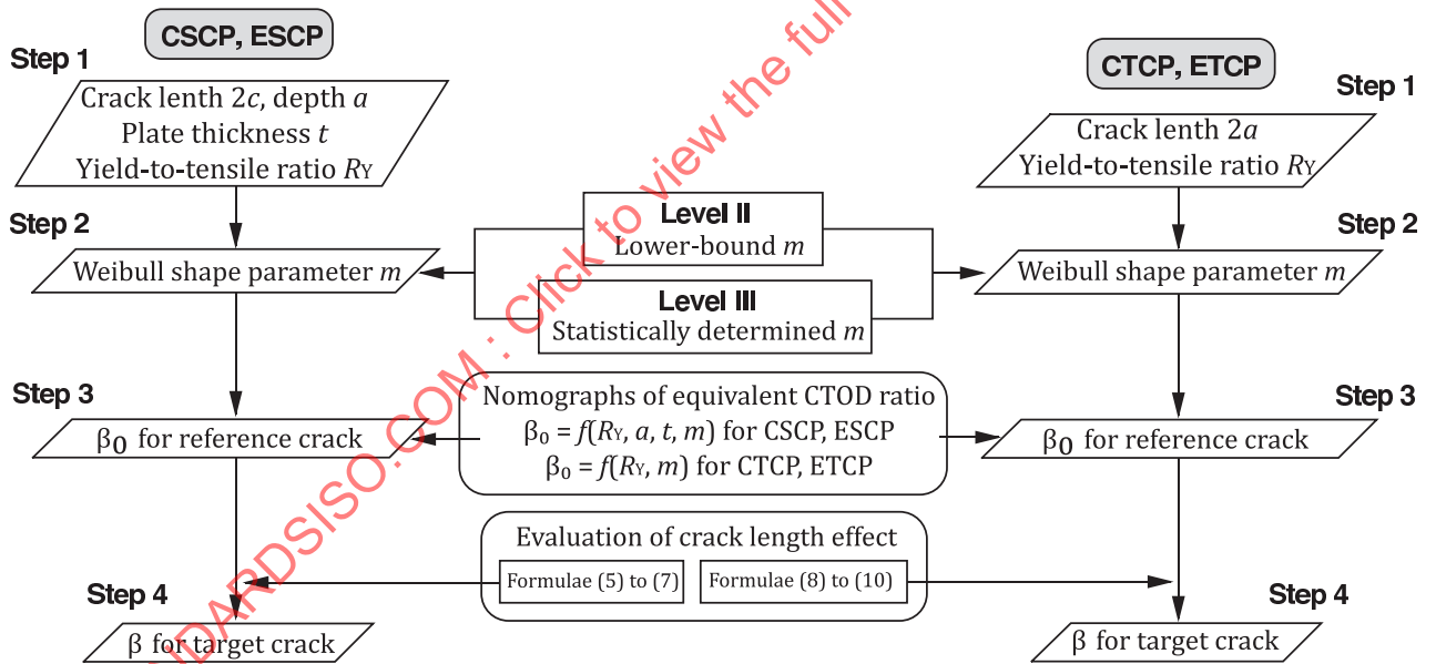
Figure 6 — Flow chart for calculating the equivalent CTOD ratio, \beta
