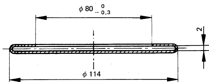
FIGURE 3 — Protective envelope
