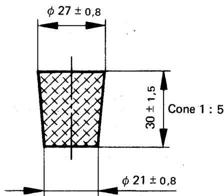
FIGURE 6 – Stopper
