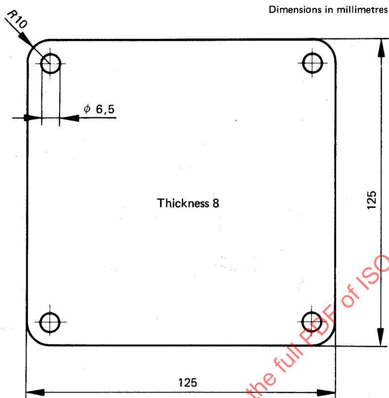
FIGURE 4 – Frame plate
