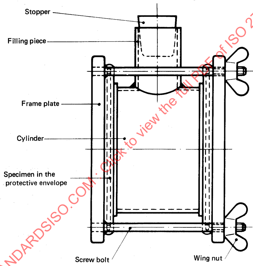
FIGURE 1 – Testing apparatus
