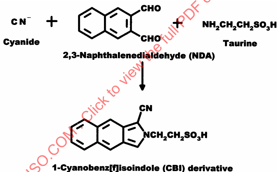
Figure 4 — Reaction of cyanide ion ( \text{CN}^- ) with 2,3-naphthalenedialdehyde (NDA) and taurine, producing 1-cyanobenz[f]isoindole [1-cyano-2-benzisoindole (CBI)] derivative
