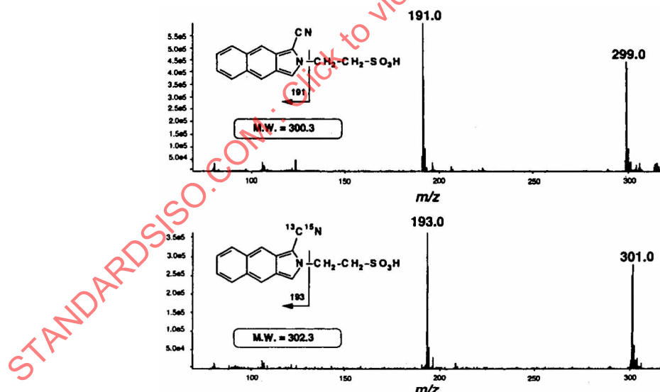
Figure B.2 — High-performance liquid chromatography — Negative-ion ion spray mass spectra of the CBI derivatives ( m/z 70 to 320) 7)
