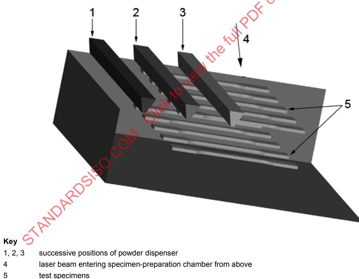
Figure A.1 — View of the interior of the specimen-preparation chamber in a laser-sintering machine
