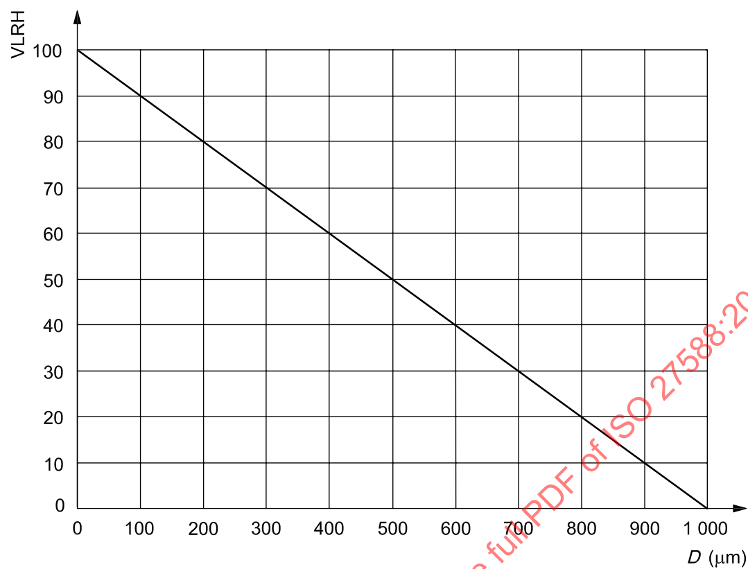
Figure A.1 — Relationship between the depth of penetration, D , and VLRH
