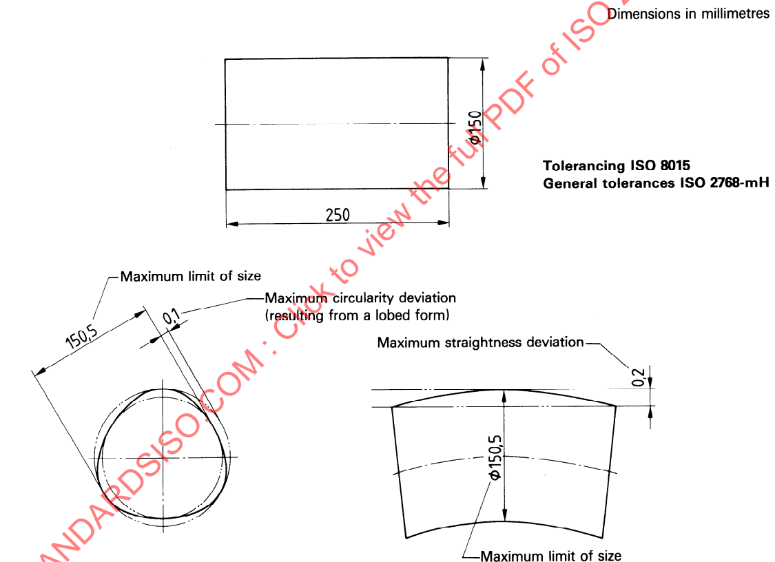
Figure B.1 — Principle of independency; maximum permissible deviations on the same feature
