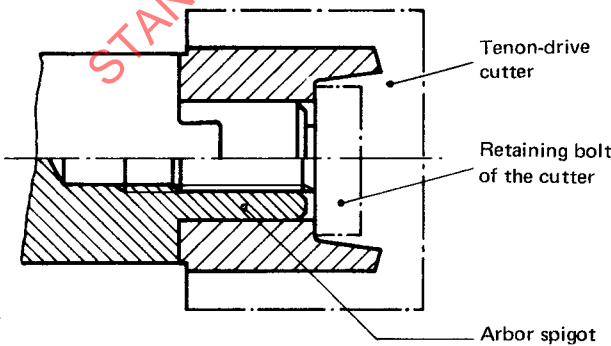
FIGURE 1 – General arrangement
