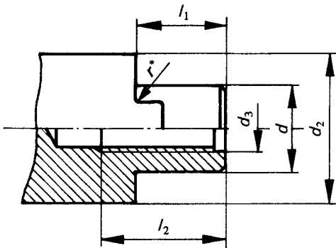
FIGURE 3 — Arbor spigot
