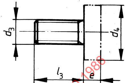
Figure 4 — Retaining bolt
