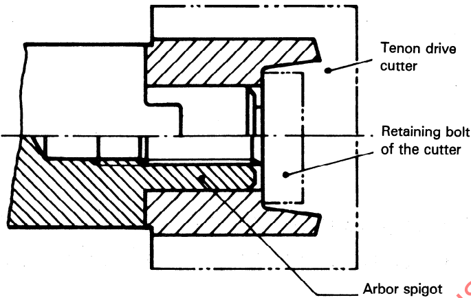
Figure 1 — General layout
