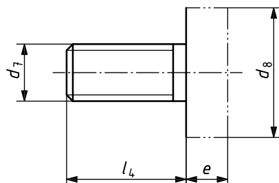
Figure 4 — Cutter retaining screw on cutter arbor
