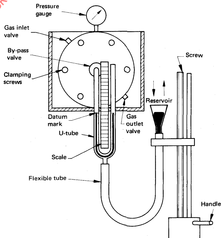
FIGURE 2 — Apparatus with vertical measuring device
