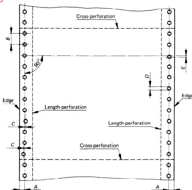
FIGURE — Sprocket feed holes
