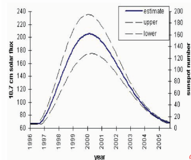
Figure 6 — Solar flux estimated upper, lower and representative trends
