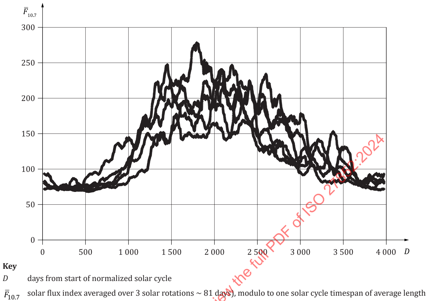
Figure 15 — \bar{F}_{10.7} Bar normalized to average cycle
