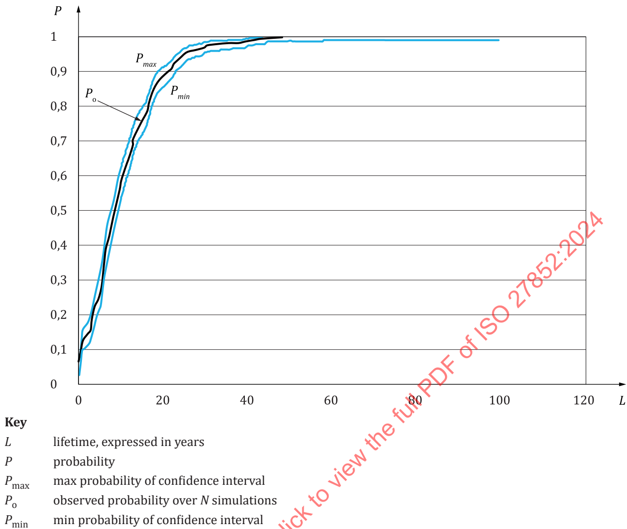
Figure 9 — Example of cumulative distribution function of orbital lifetimes with a 95 % confidence interval (500 runs)
