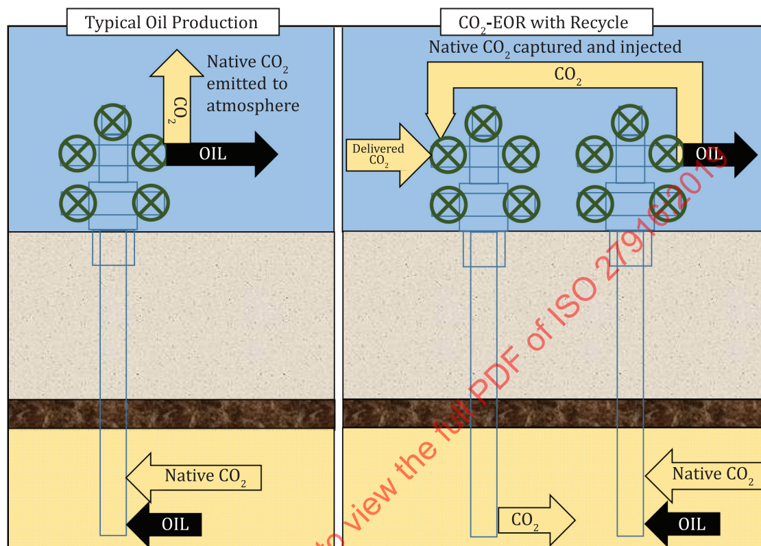
Figure 1 — Illustration of native CO 2 previously being emitted with typical production and now being captured and injected with CO 2 -EOR (This diagram is to show movement of native CO 2 only and not meant to demonstrate production of other sources of CO 2 )
