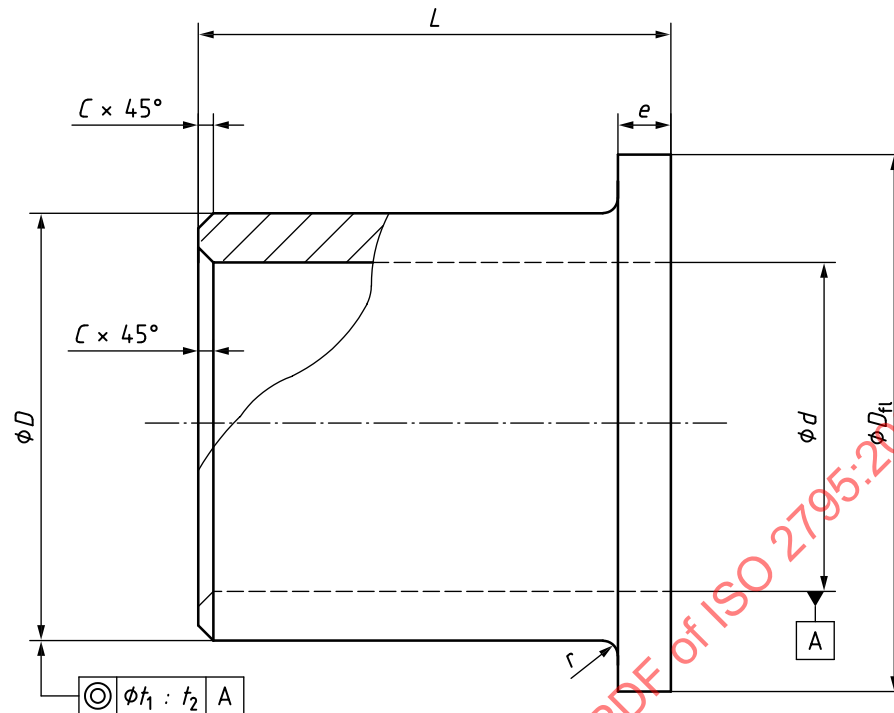
Figure 2 — Flanged bearing
