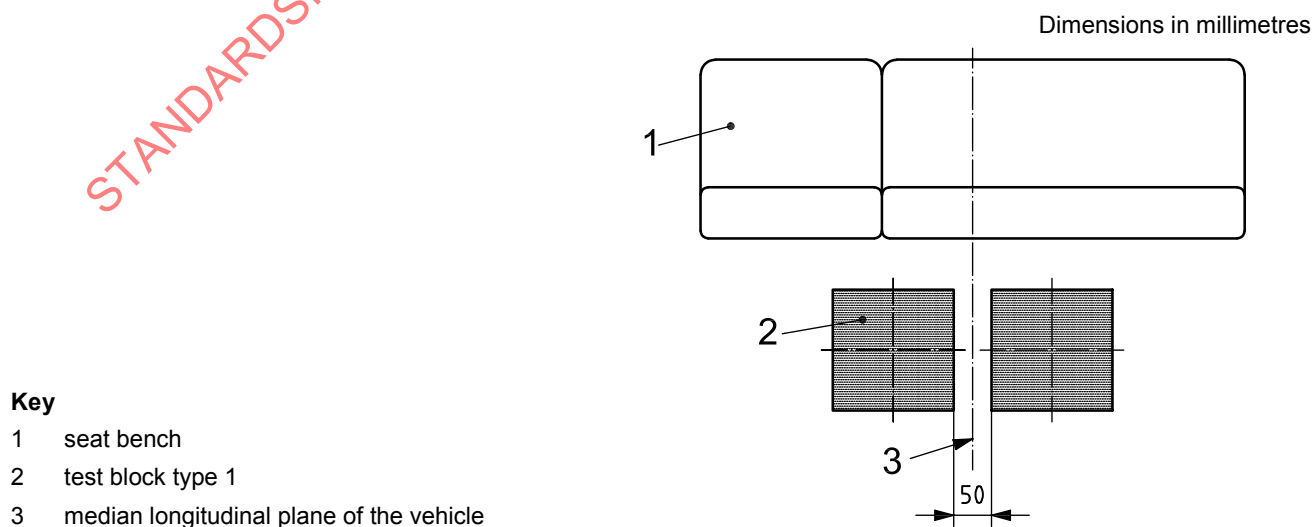
Figure 9 — Testing of a combination of a single seat and a seat bench (normally a rear-seat bench)
