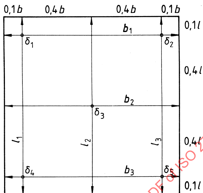
Figure — Positions for measuring dimensions
