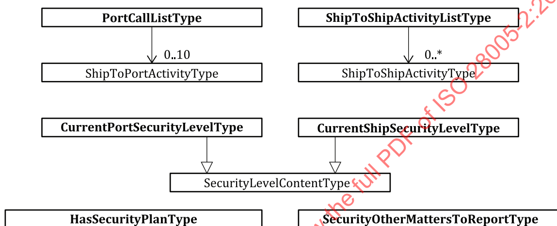
Figure 7 — Security related data items
