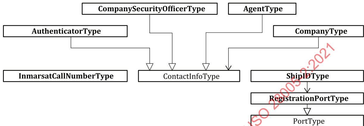
Figure 3 — Class diagram for ship identity and contact details
