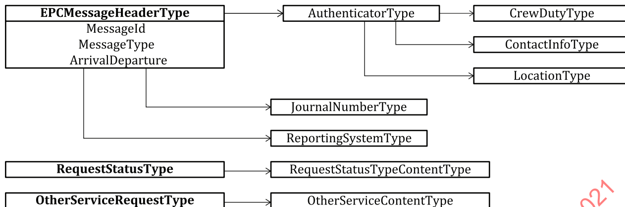
Figure 8 — Services data types class diagram
