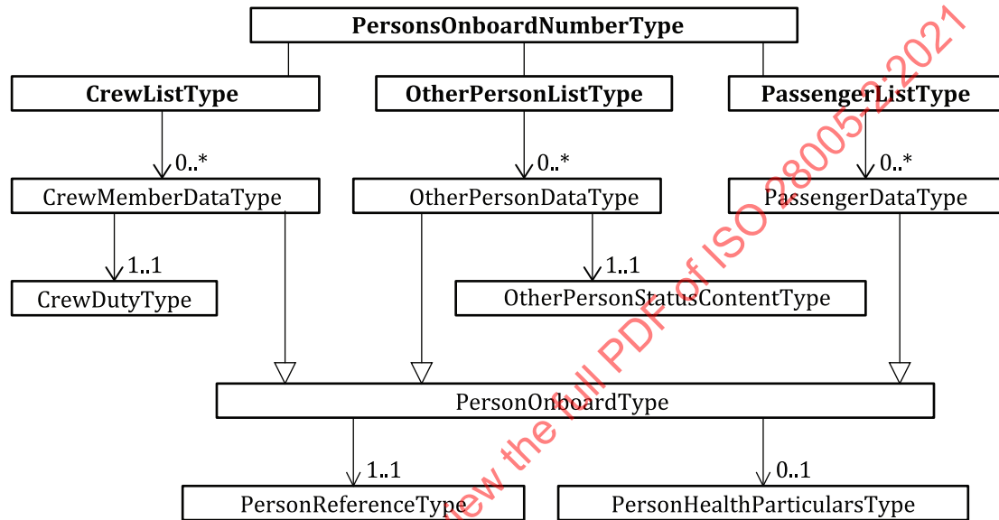
Figure 5 — Crew and passenger class diagram
