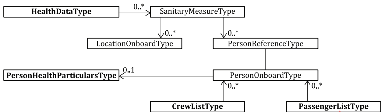
Figure 10 — Health data items
