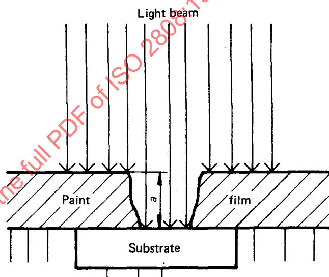
FIGURE 3 — Sectioned view of incised painted specimen
