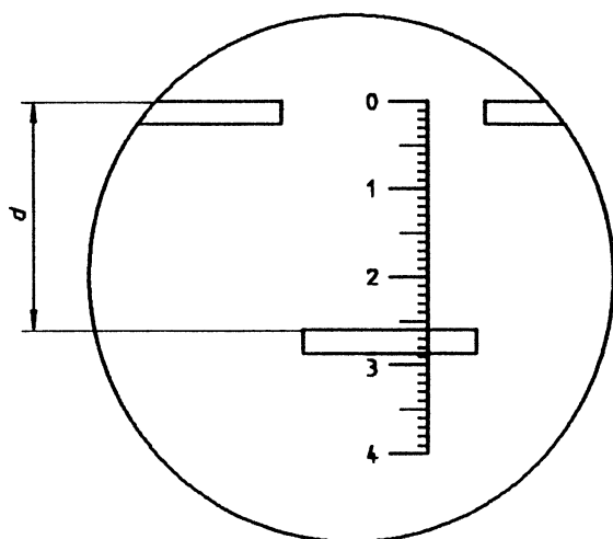
Figure 4 — Typical image as seen in the microscope
