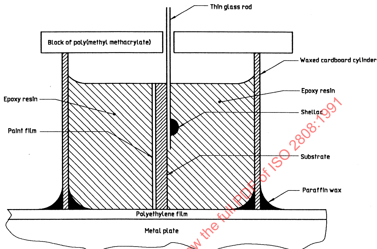
Figure 1 — Method of preparing specimens for measurement of dry film thickness according to microscope method 5A
