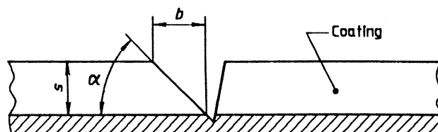
Figure 2 — Diagrammatic representation of the wedge cut
