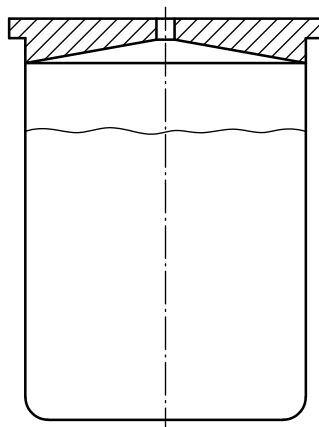
Figure 1 — Metal pyknometer
