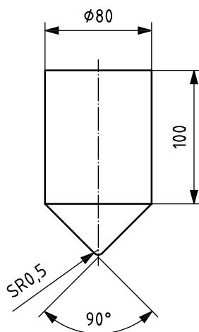
Figure 1 — Test cone
