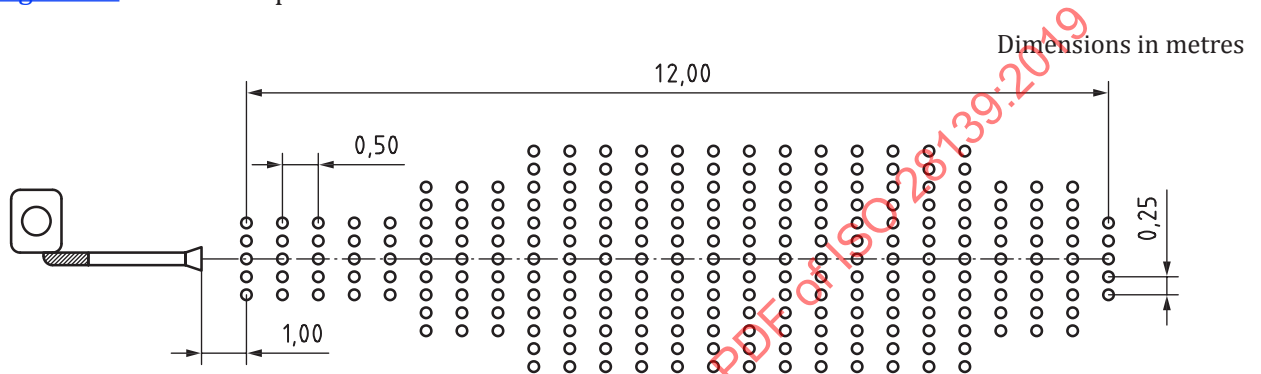
Figure F.1 — Example of sprayer and Petri dish positioning
