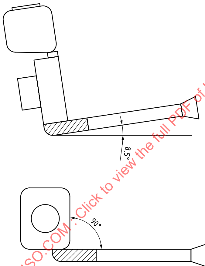
Figure C.1 — Position of sprayer for stability testing
