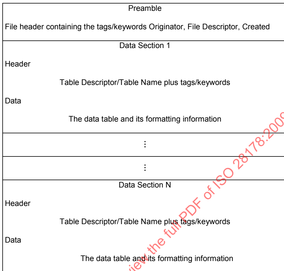
Figure 1 — File structure
