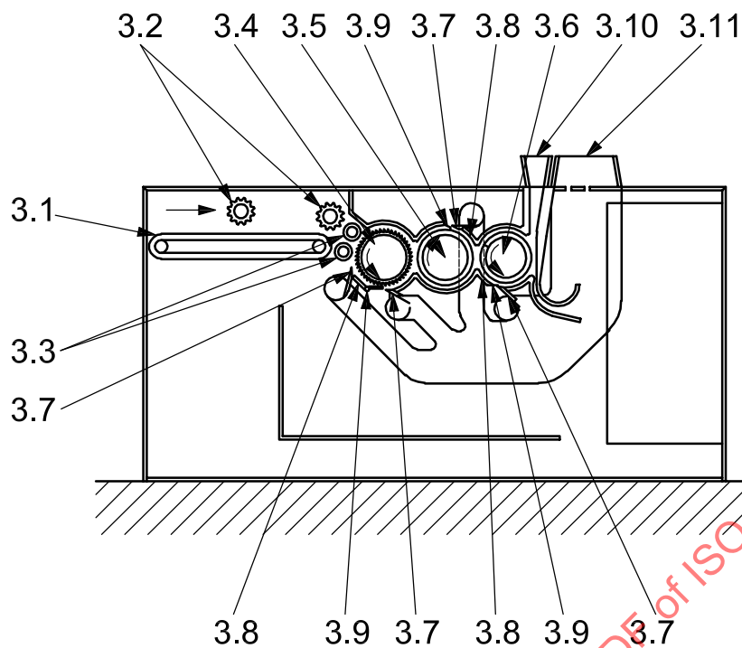
Figure 3 — Machine components — Cleaner
