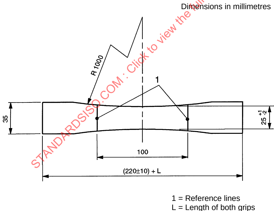
Figure 3 - Type A test piece
