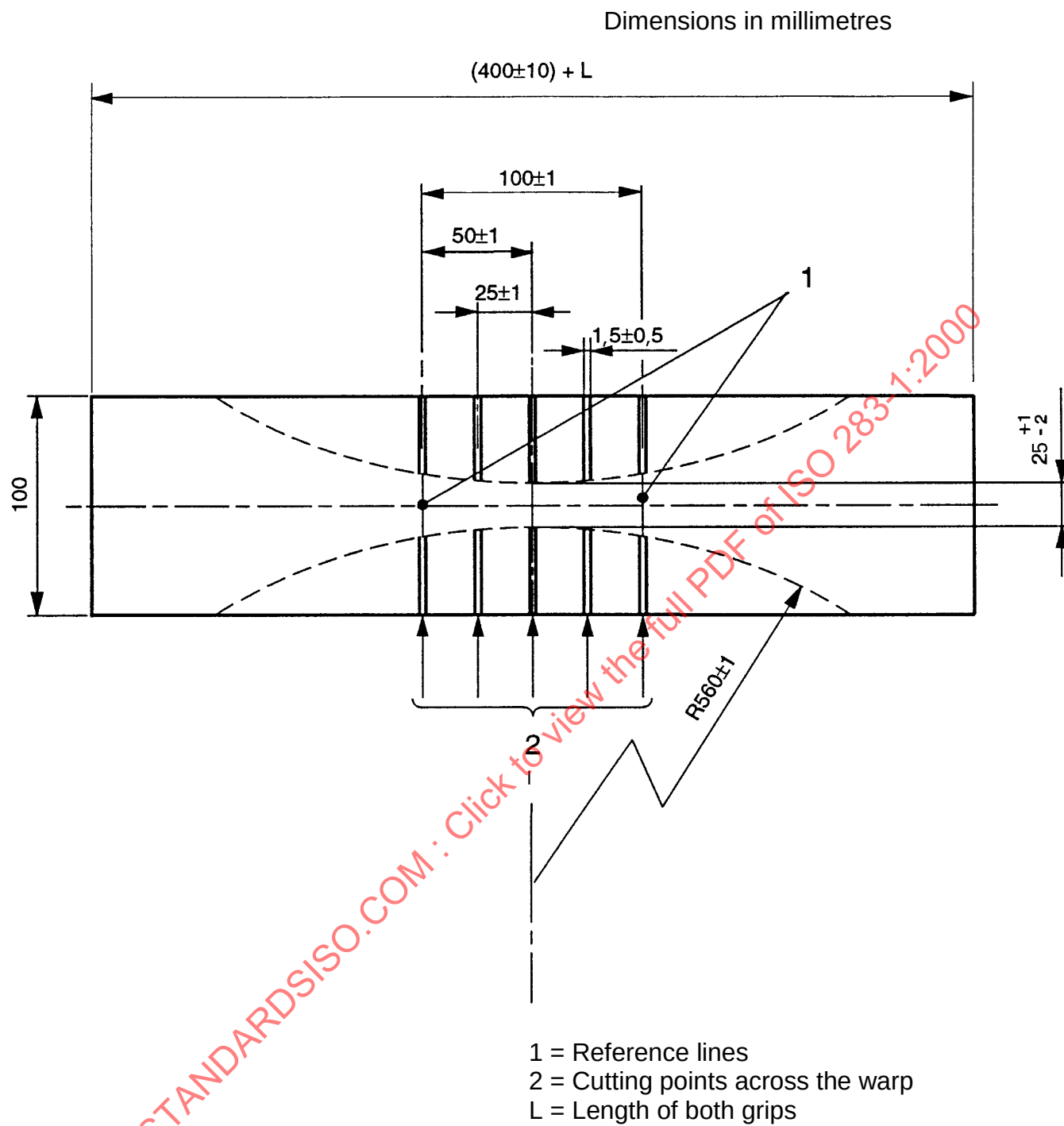
Figure 6 - Type D test piece
