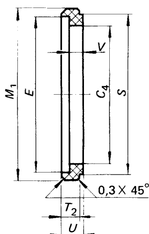
Gasket to be used with the support ring in clause 12
