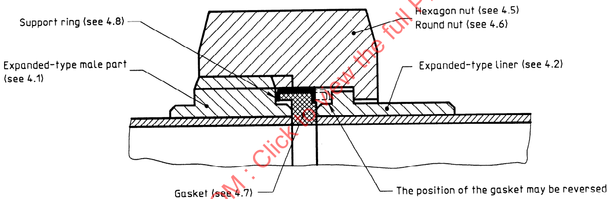
Figure B.1 — Expanded-type coupling
